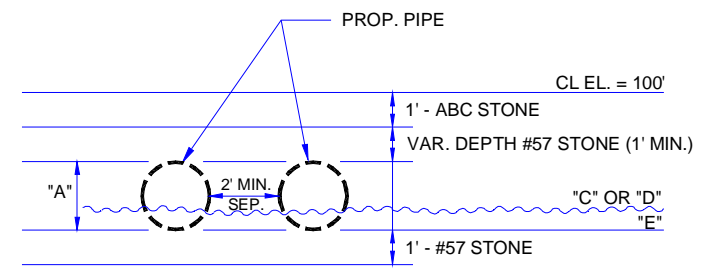
SECTION VIEW NTS
