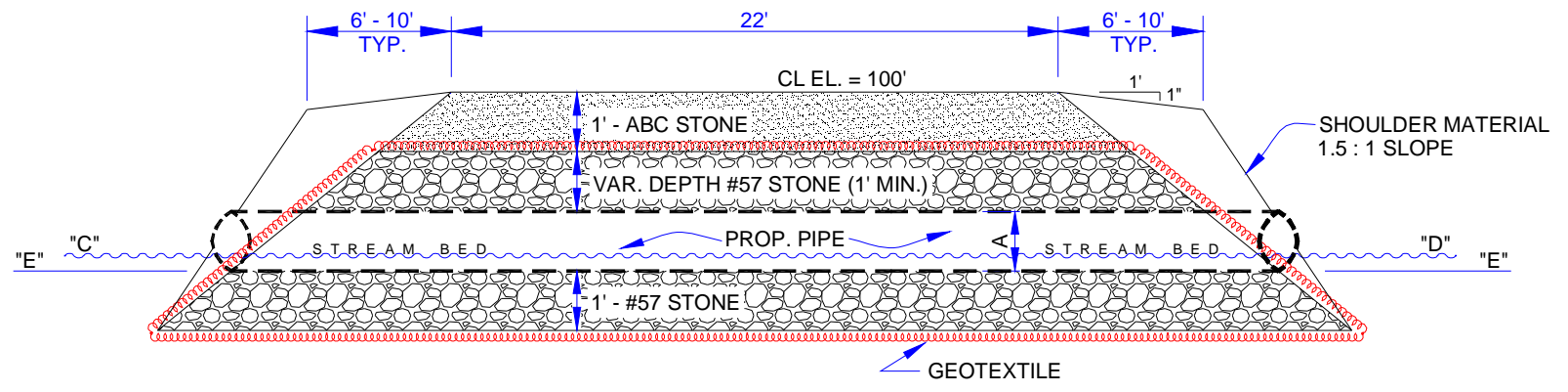
SECTION VIEW NTS
